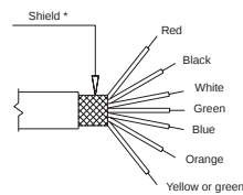
6x0.25 Screened cable
