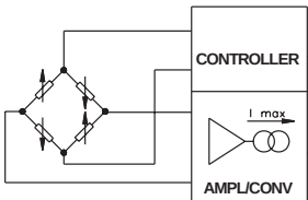
CURRENT AMPLIFIED OUTPUT - mod. E
