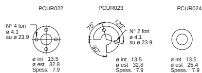
Floating magnets
